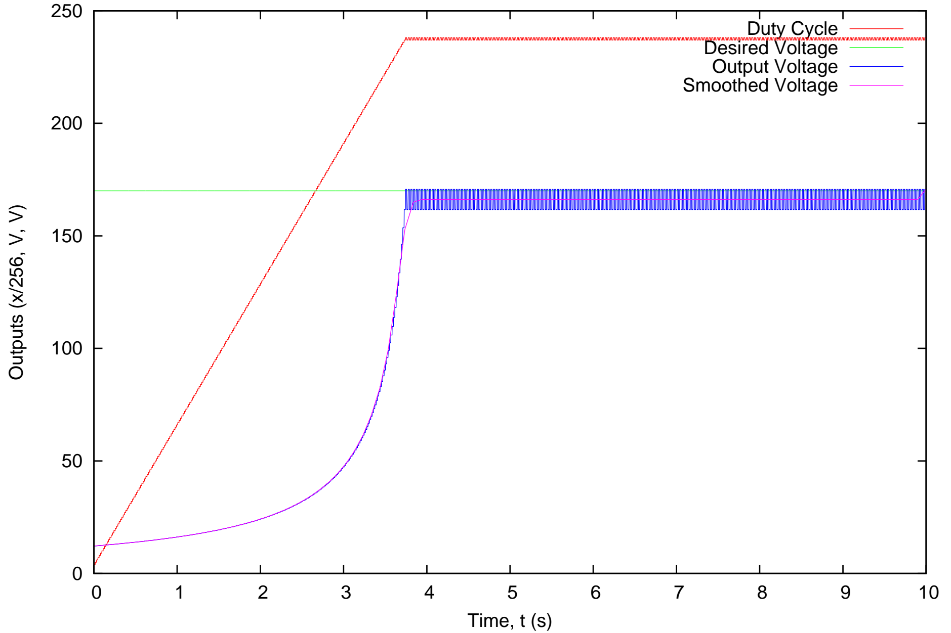
Boost Converter 1.0 - System Outputs
