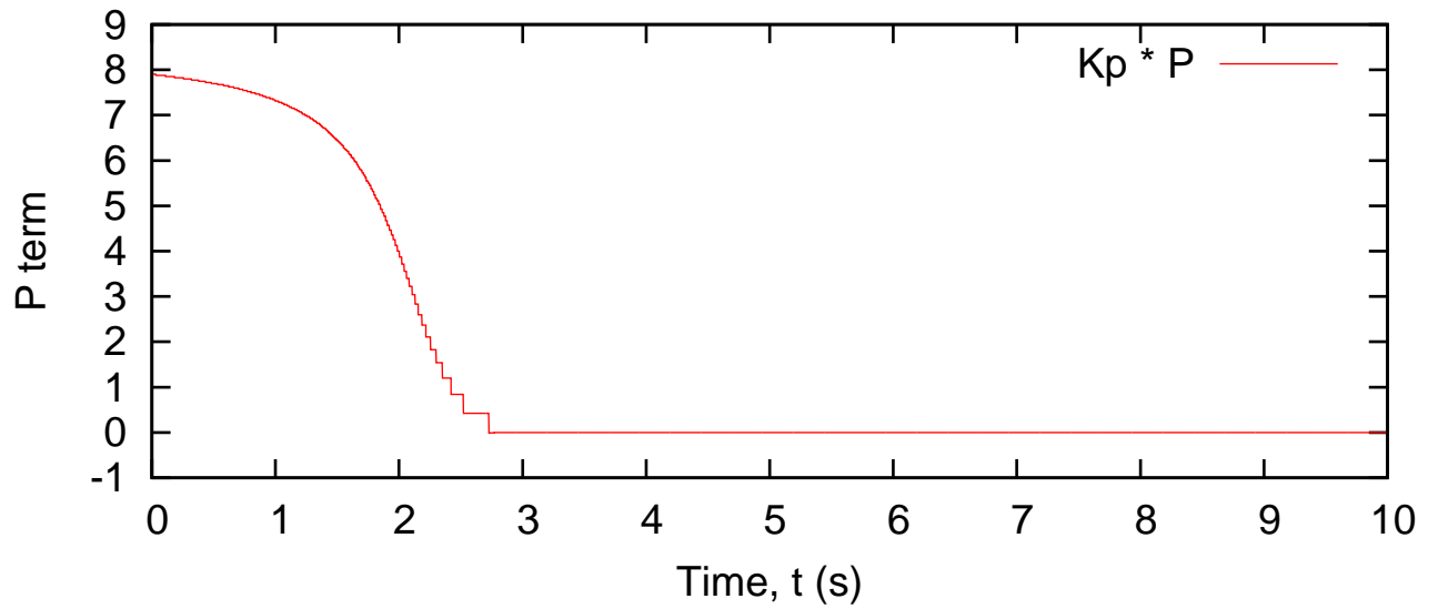
PID Boost Converter - Proportional term
