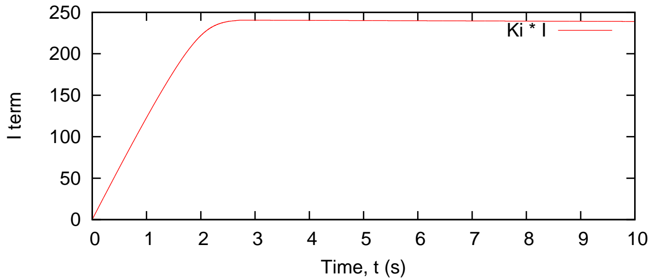
PID Boost Converter - Integral term
