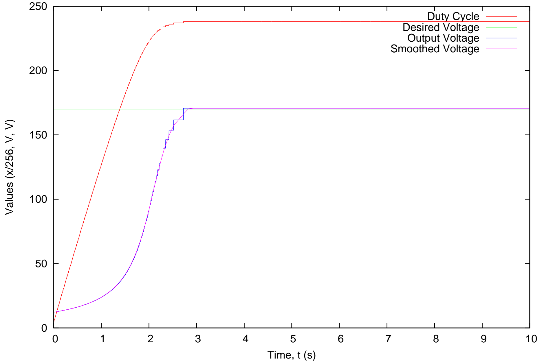
PID Boost Converter - System Outputs
